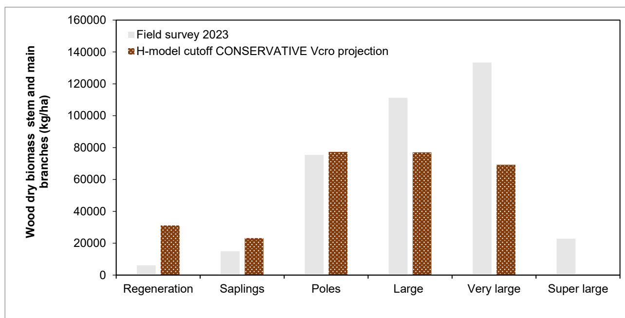
Figure 8. Estimated wood dry biomass per hectare per silvicultural class in the survey and in the HMCC.
