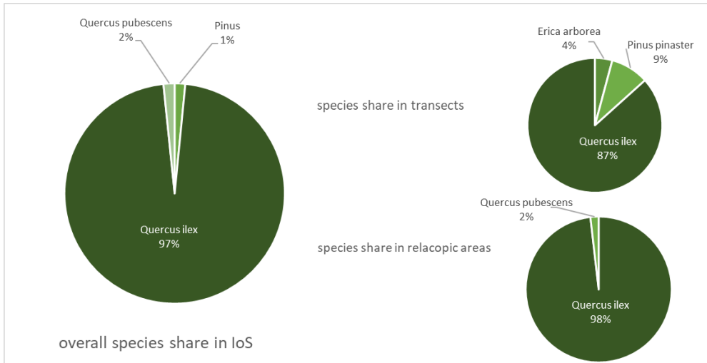
Figure 9. Species share in IB 2023.
