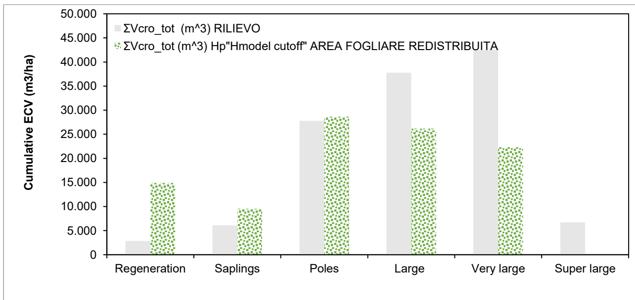
Figure 7. Estimated crown volume per hectare per silvicultural class in the survey and in the HMCC.
