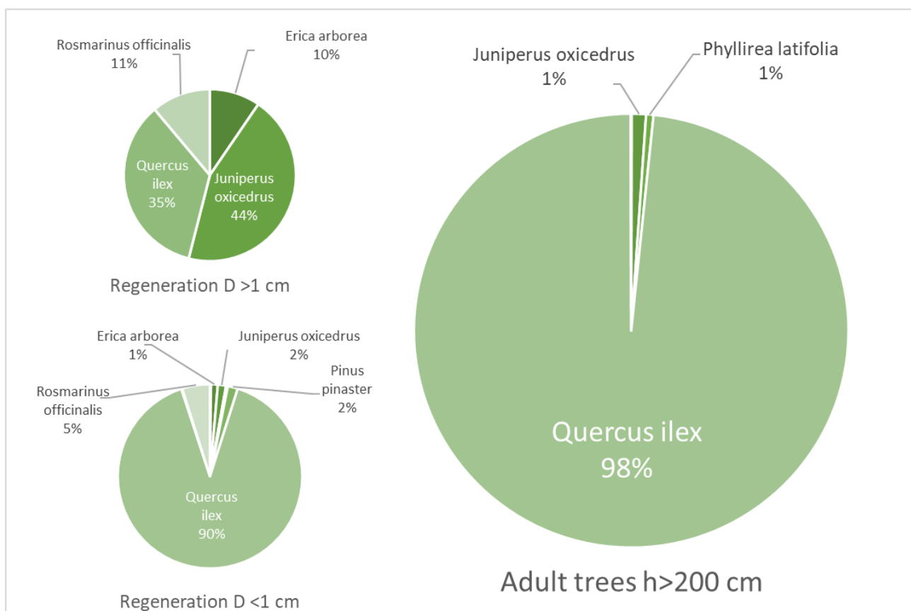
Figure 1. Species share in Montes Forest 2023.
