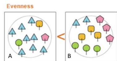
Figure 1. Graphs A and B display the same species richness. However, Graph B shows a more even distribution of individuals among species, resulting in a higher evenness index compared to Graph A.
